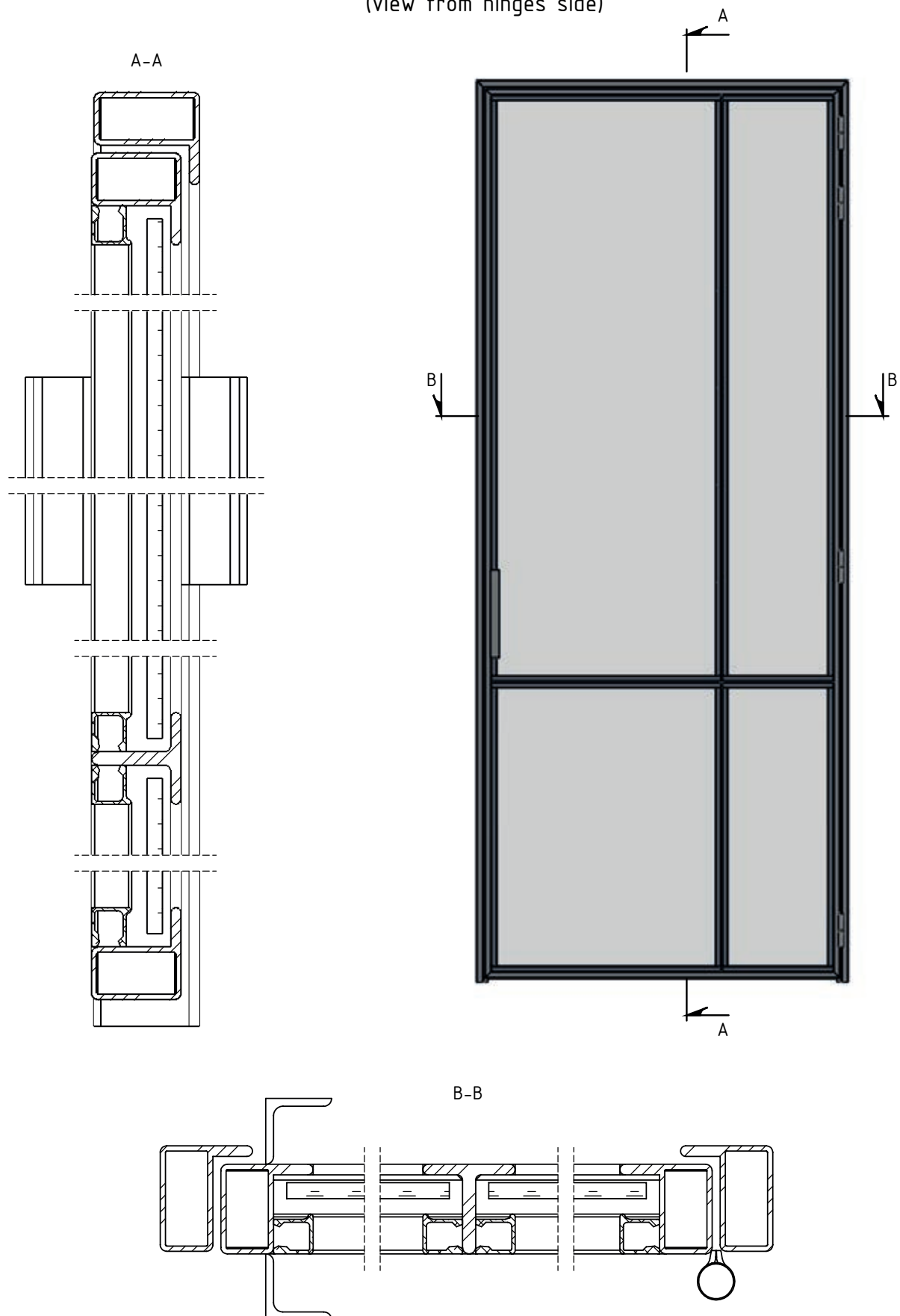
40 line RP (view from hinges side)
