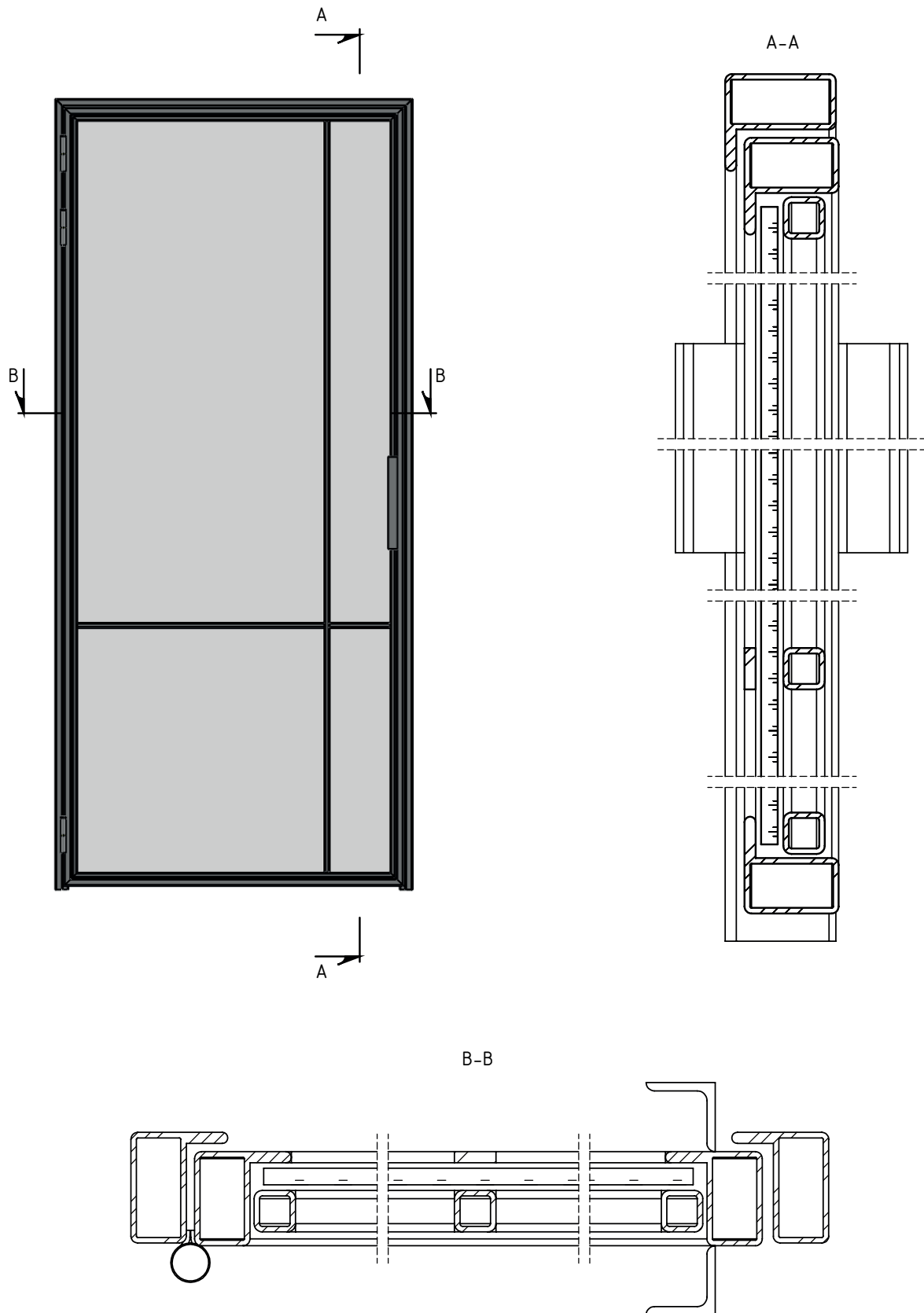
40 line tube (view from hinges side)
