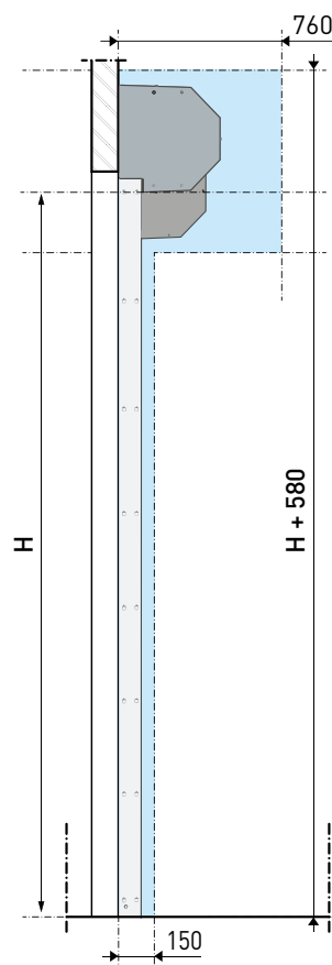
[ Dwarsdoorsnede ]
