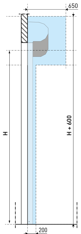
[ Dwarsdoorsnede ]
