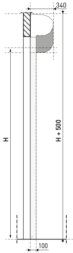
[ Dwarsdoorsnede ]
