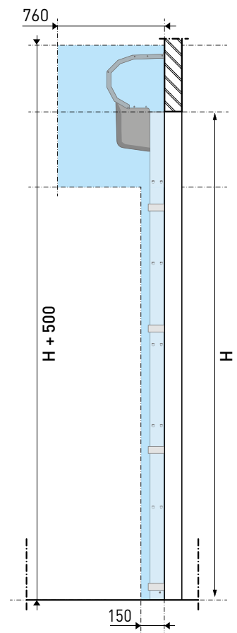
— [ Dwarsdoorsnede ] —
